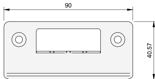
STRIKE PLATE (GLASS DOOR) S9SPG
