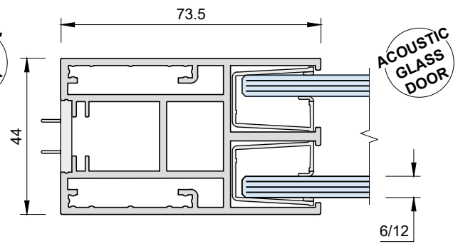
ALUMINIUM DOUBLE GLAZED DOOR PLUS
