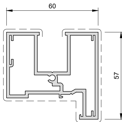
CENTRE GLAZED DOOR FRAME S9SCGFRAME (TO SUIT STANDARD DOOR SIZES)
