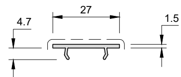
CLIP IN COVER
