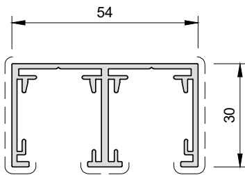
30mm DEEP HEAD CHANNEL S9NGHEAD ●
