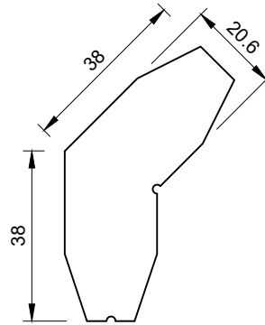
135° TRACK CLEAT S9CLEAT135
