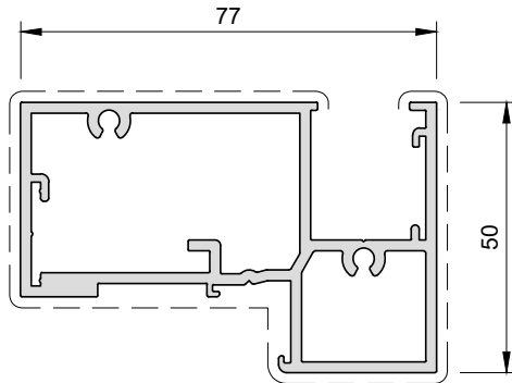
OFFSET GLAZED DOOR FRAME S9SGFRAME (TO SUIT STANDARD DOOR SIZES)
