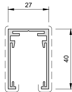
40mm DEEP HEAD CHANNEL S9SGHEAD40 ●
