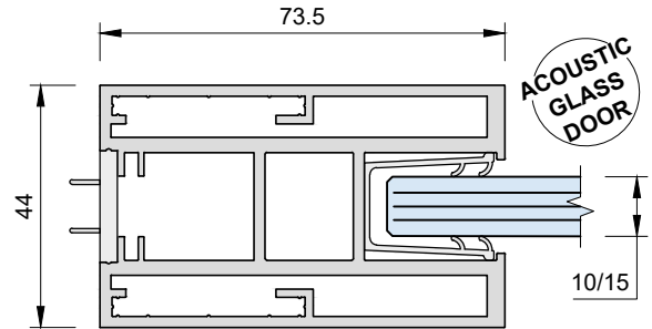
ALUMINIUM SINGLE GLAZED DOOR
