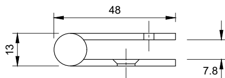
FIXED PIN DOOR HINGE (USE WITH TIMBER DOORS) PTH103
