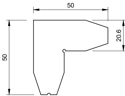
90° TRACK CLEAT S9CLEAT90
