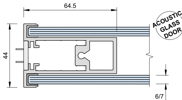
ALUMINIUM DOUBLE GLAZED DOOR
