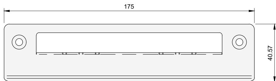
STRIKE PLATE (TIMBER DOOR) S9SPT
