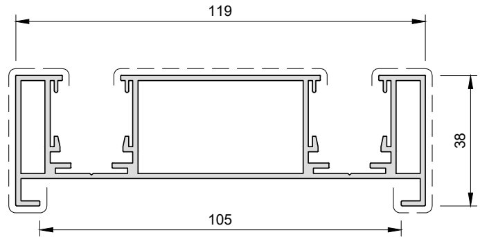
DRYWALL / INTEGRATION POST
