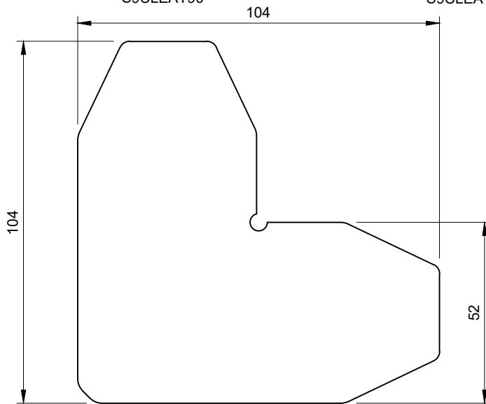
90° (CENTRAL POCKET) DOOR FRAME CLEAT S9CPDCLEAT90
