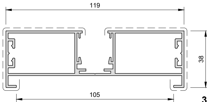
DRYWALL / INTEGRATION POST (SINGLE GLAZED) S9SGIP ●
