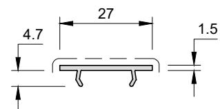
CLIP IN COVER S9CIC ●
