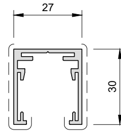
30mm DEEP HEAD CHANNEL S9SGHEAD30 ●
