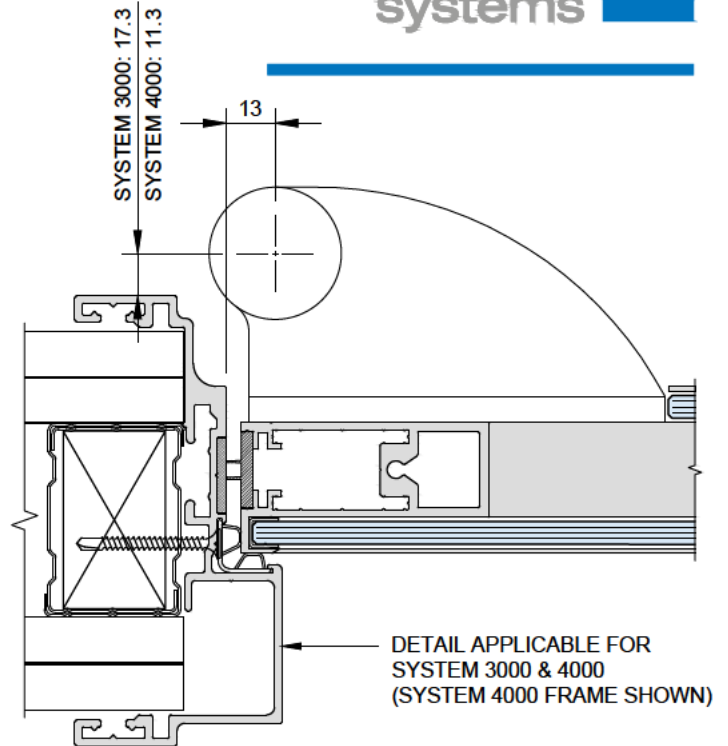
02 SYSTEM 3000/4000 DOOR FRAME Scale: 1:2
