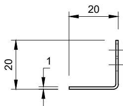
GHOST POST BRACKET S9GPB
