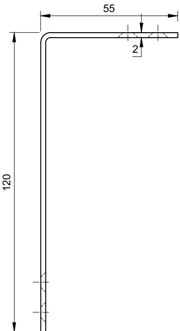
CORNER BRACKET S9CB
