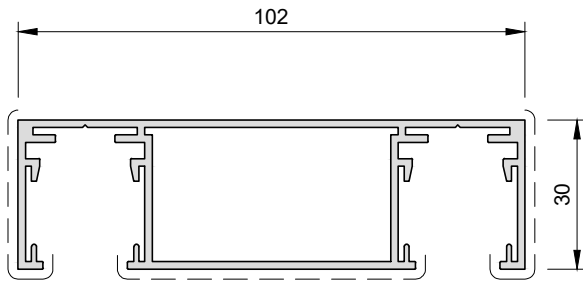
30mm DEEP HEAD CHANNEL
