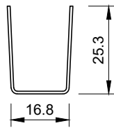
STEEL CLIP IN CAPPING SECTION
