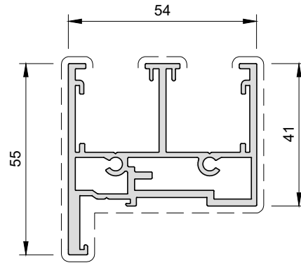
DOOR FRAME S9NGFRAME (TO SUIT STANDARD DOOR SIZES)
