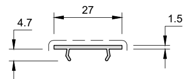
CLIP IN COVER S9CIC ●
